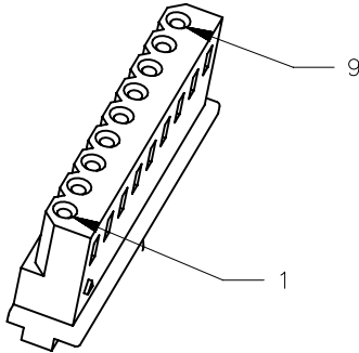
P2 PIN DESIGNATION SCALE 2:1
