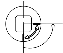
OPTION 2 FOR INSTALLATION OF ROTATION LIMITER - VIEWED FROM BACK-
