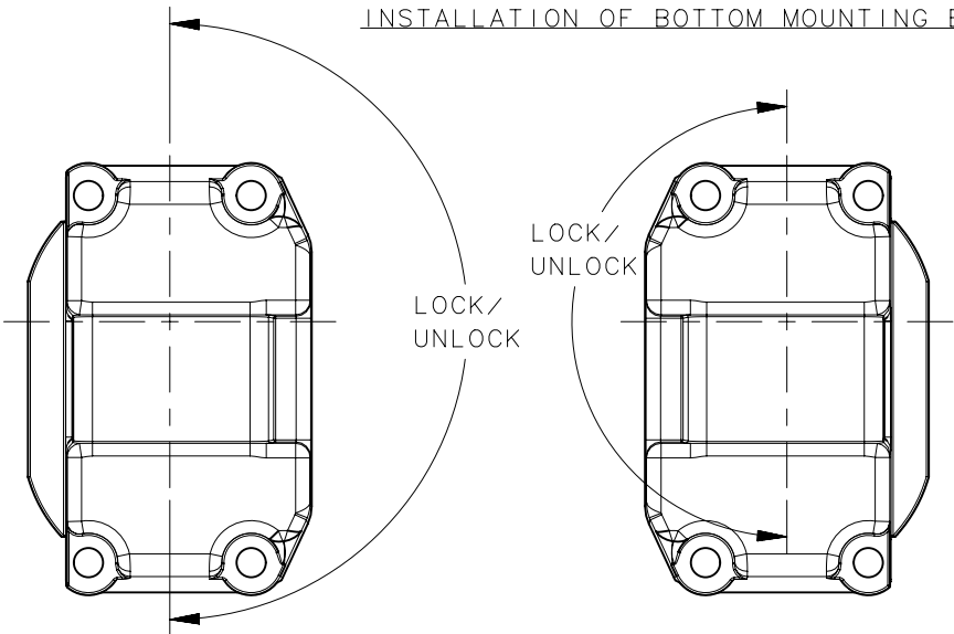
INSTALLATION OF BOTTOM MOUNTING BRACKET
