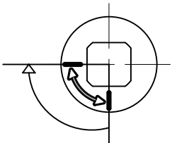
OPTION 1 FOR INSTALLATION OF ROTATION LIMITER - VIEWED FROM BACK-
