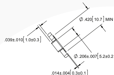
OPENED POSITION (AS MOLDED)
